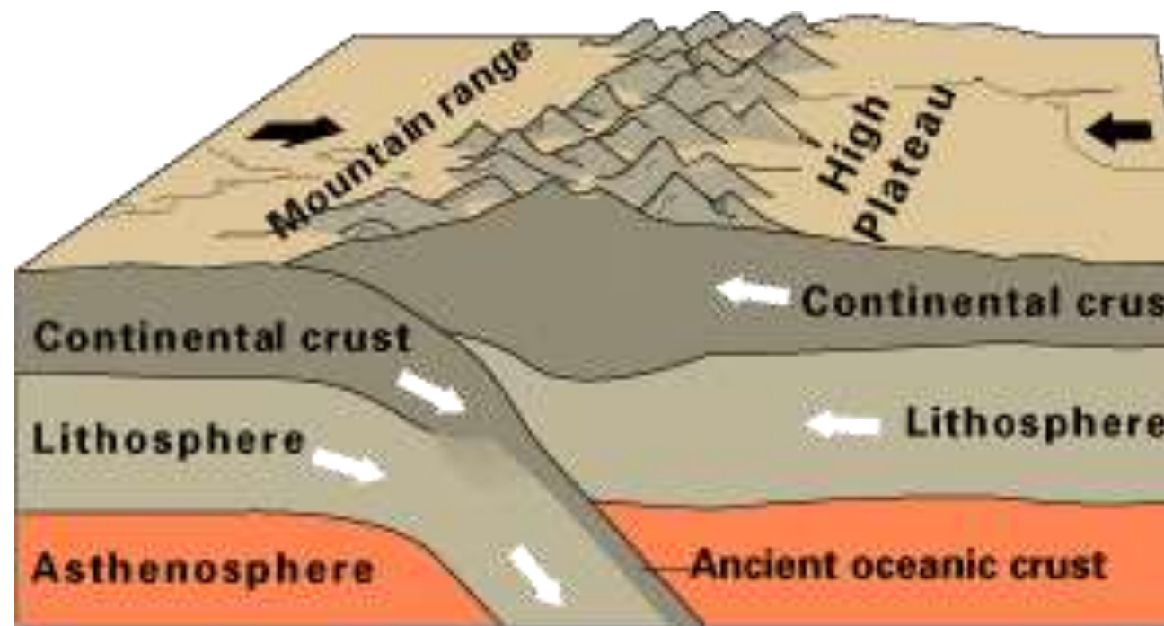
Continental-continental convergence
